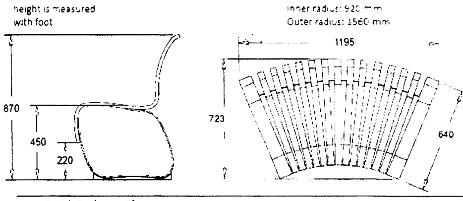
Nova C with Backrest 45° concave
