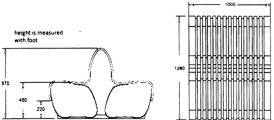
Nova C with Backrest double straight
