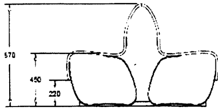
Nova C with Backrest double 45° concave
