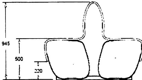
Nova Senior double straight
